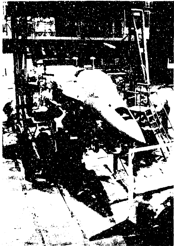
FIG. 38 - STRUCTURAL TESTS
