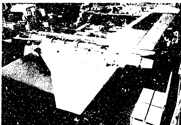
FIG. 22 - RAFALE - FULL SCALE LAYOUT MOCK-UP
